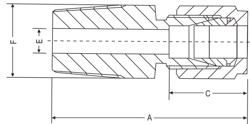
Dimensional Details :
